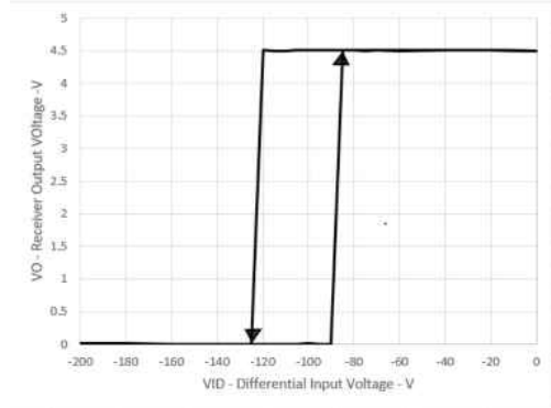
图 5-6. Receiver Output Voltage vs Differential Input Voltage
