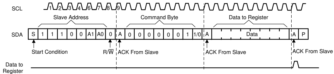
图 7-9. Write To Configuration Or Polarity Inversion Registers
