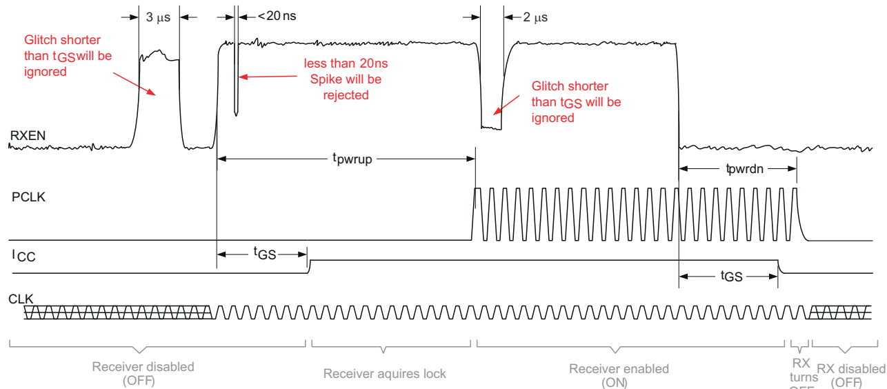
图 7-10. Receiver Enable and Disable Glitch Suppression Time
