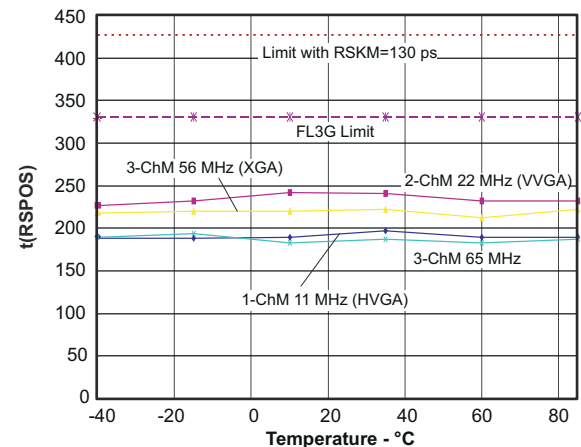
图 6-6. Receiver Strobe Position vs Temperature
