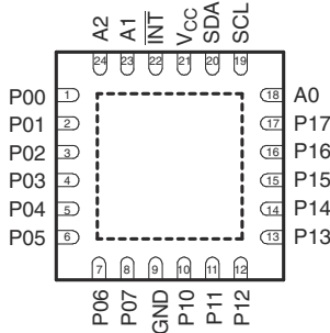
RTW PACKAGE (TOP VIEW)
