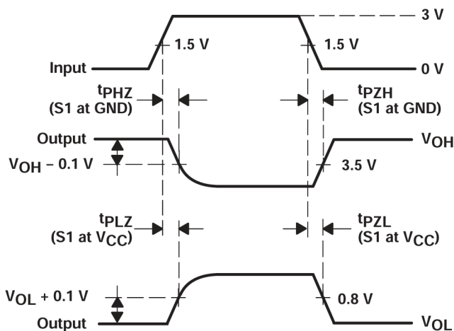
VOLTAGE WAVEFORMS
