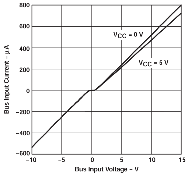
图 5-1. Bus Input Current vs Bus Input Voltage
