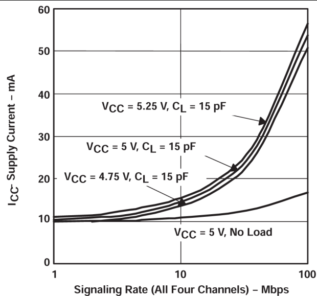
图 5-3. Supply Current vs Signaling Rate (All Four Channels)
