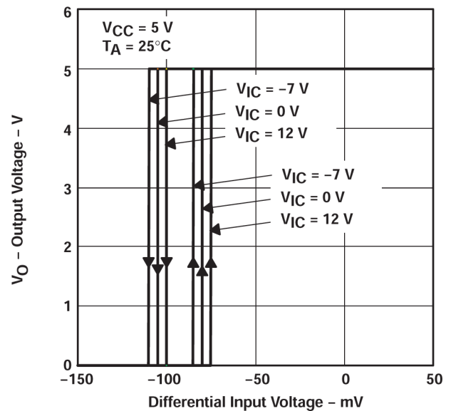
图 5-2. Output Voltage vs Differential Input Voltage
