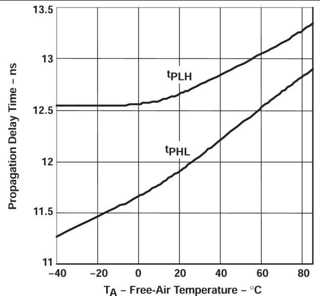
图 5-4. Propagation Delay Time vs Free-air Temperature
