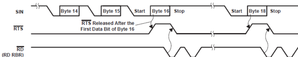
图 7-4. RTS Functional Timing Waveforms, RCV FIFO Trigger Level = 14 Bytes
