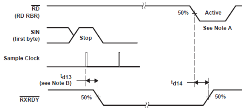
图 6-7. Receiver Ready ( \overline{\text{RXRDY}} ) Waveforms, \text{FCR0} = 0 or \text{FCR0} = 1 and \text{FCR3} = 0 (Mode 0)
