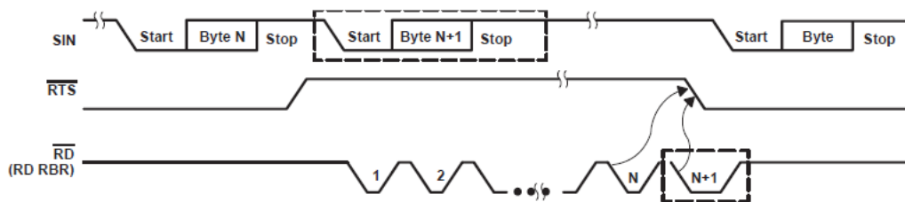
图 7-3. RTS Functional Timing Waveforms, RCV FIFO Trigger Level = 1, 4, or 8 Bytes
