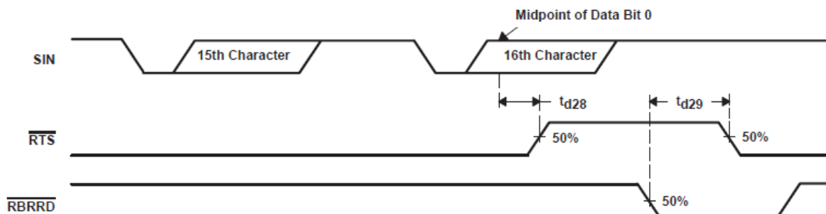
图 6-15. Auto- \overline{\text{RTS}} Timing for RCV Threshold of 14 Waveforms
