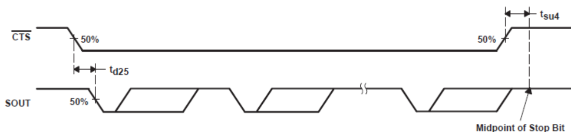
图 6-13. CTS and SOUT Autoflow Control Timing (Start and Stop) Waveforms
