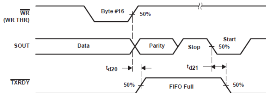
图 6-11. Transmitter Ready (TXRDY) Waveforms, FCR0 = 1 and FCR3 = 1 (Mode 1)
