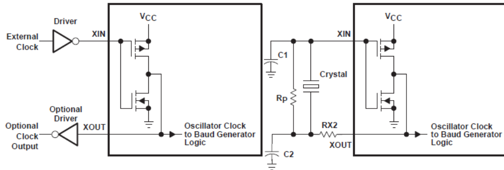
图 7-5. Typical Clock Circuits
