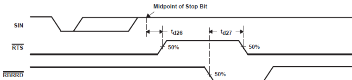
图 6-14. Auto- \overline{\text{RTS}} Timing for RCV Threshold of 1, 4, or 8 Waveforms
