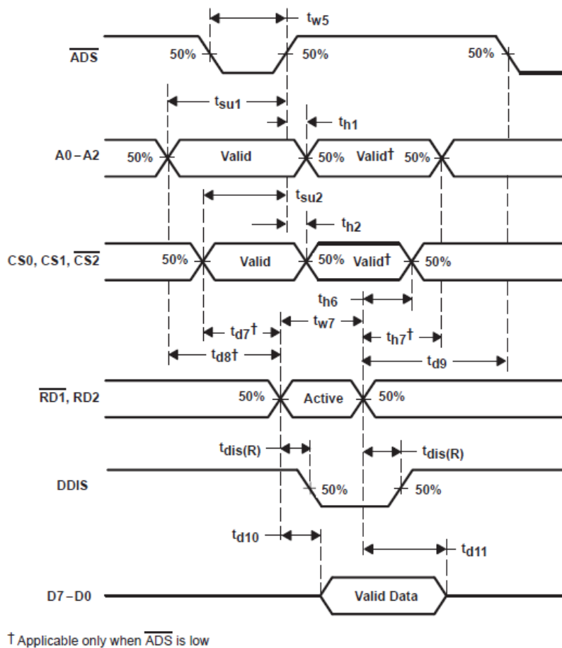
图 6-3. Read Cycle Timing Waveforms
