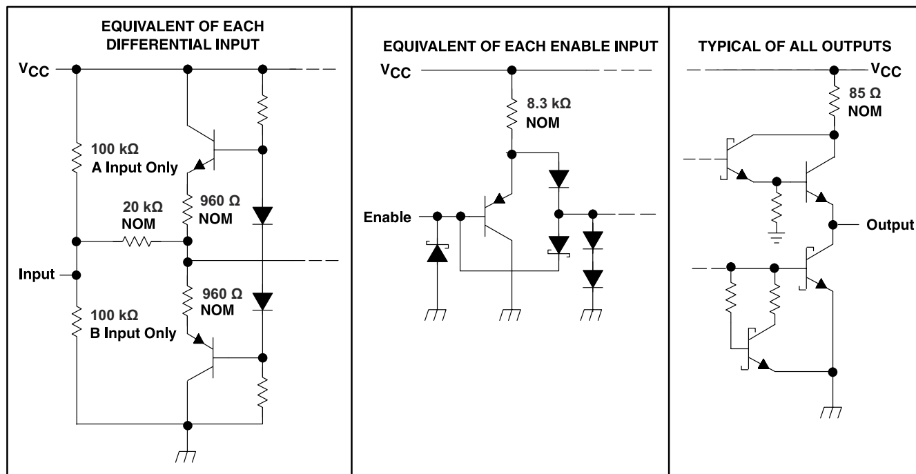
图 7-5. Schematics of Inputs and Outputs
