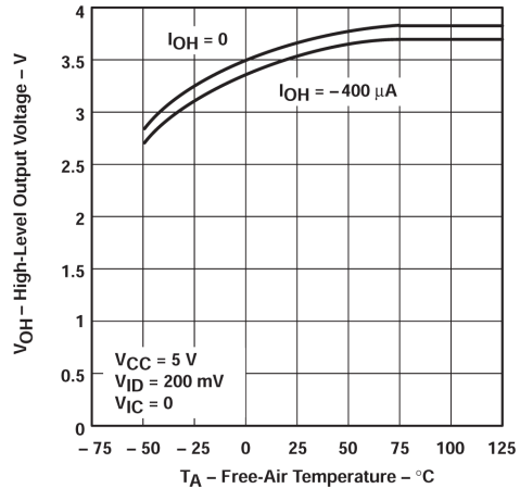
图 5-6. High-level Output Voltage vs Free-air Temperature
