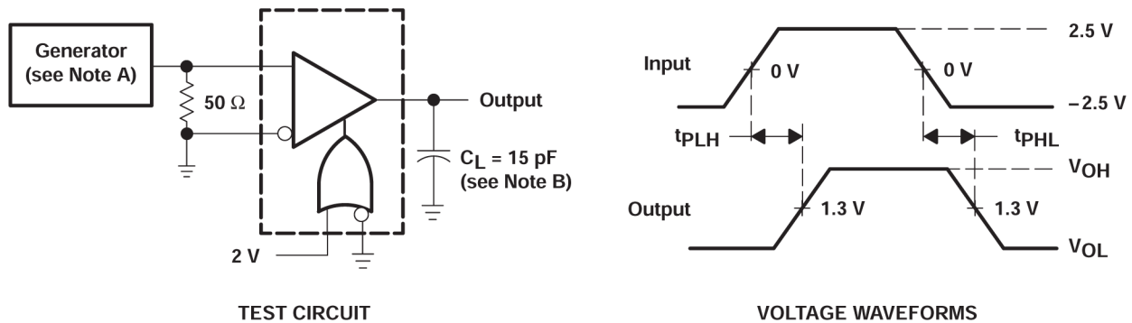
TEST CIRCUIT
