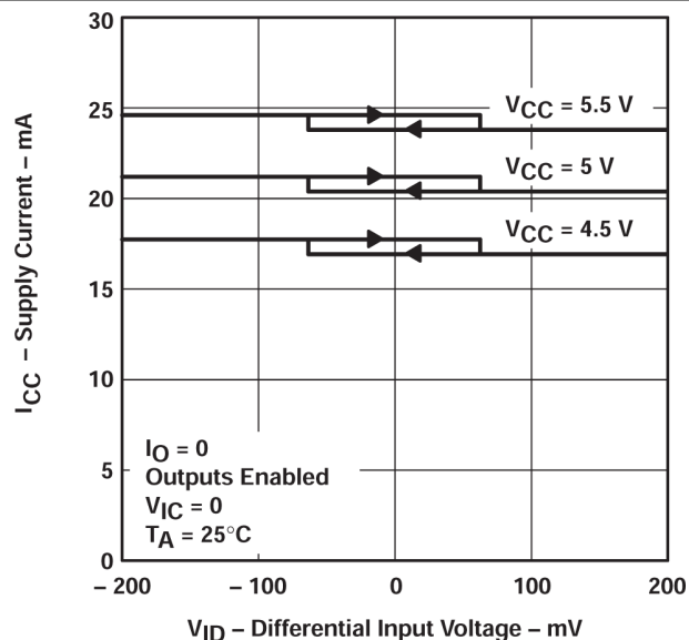
图 5-14. Supply Current vs Differential Input Voltage
