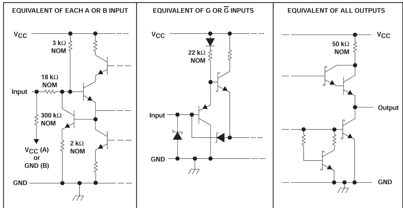
图 7-1. Schematics of Inputs and Outputs
