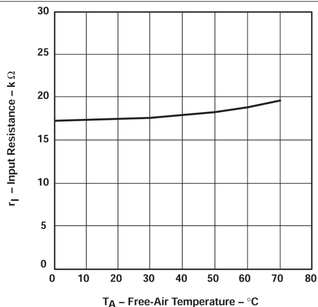
图 5-16. Input Resistance vs Free-air Temperature
