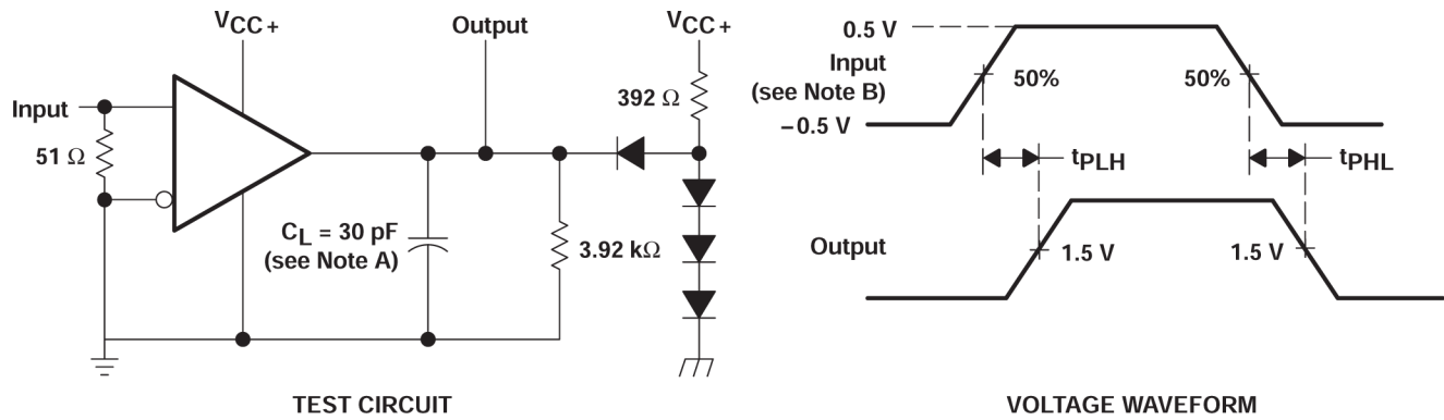
图 6-1. Test Circuit and Voltage Waveform
