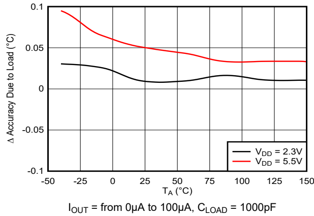
图 5-3. Changes in Accuracy vs Ambient Temperature (Due to Load)
