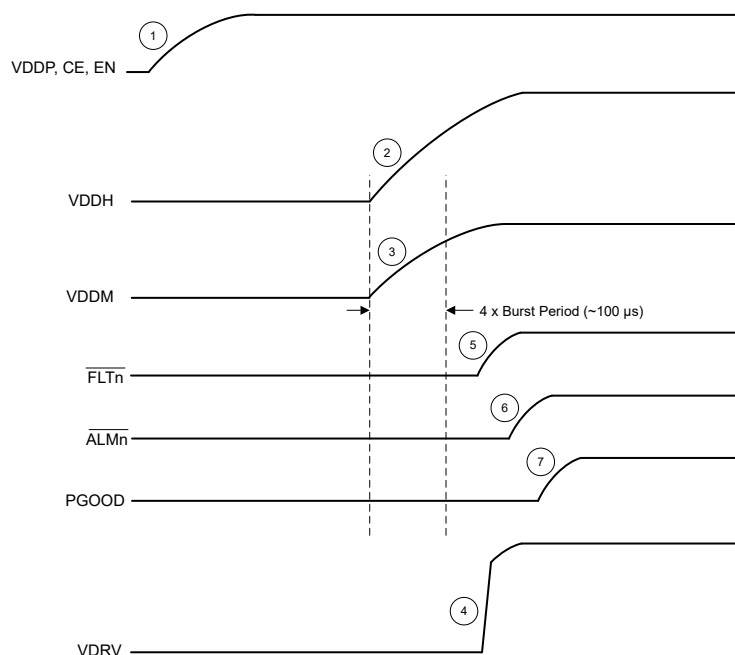
图 8-11. TPSI310x 典型启动 ( CE = EN = VDDP , FLTn\_CMP = 0 , ALMn\_CMP = 0 )
