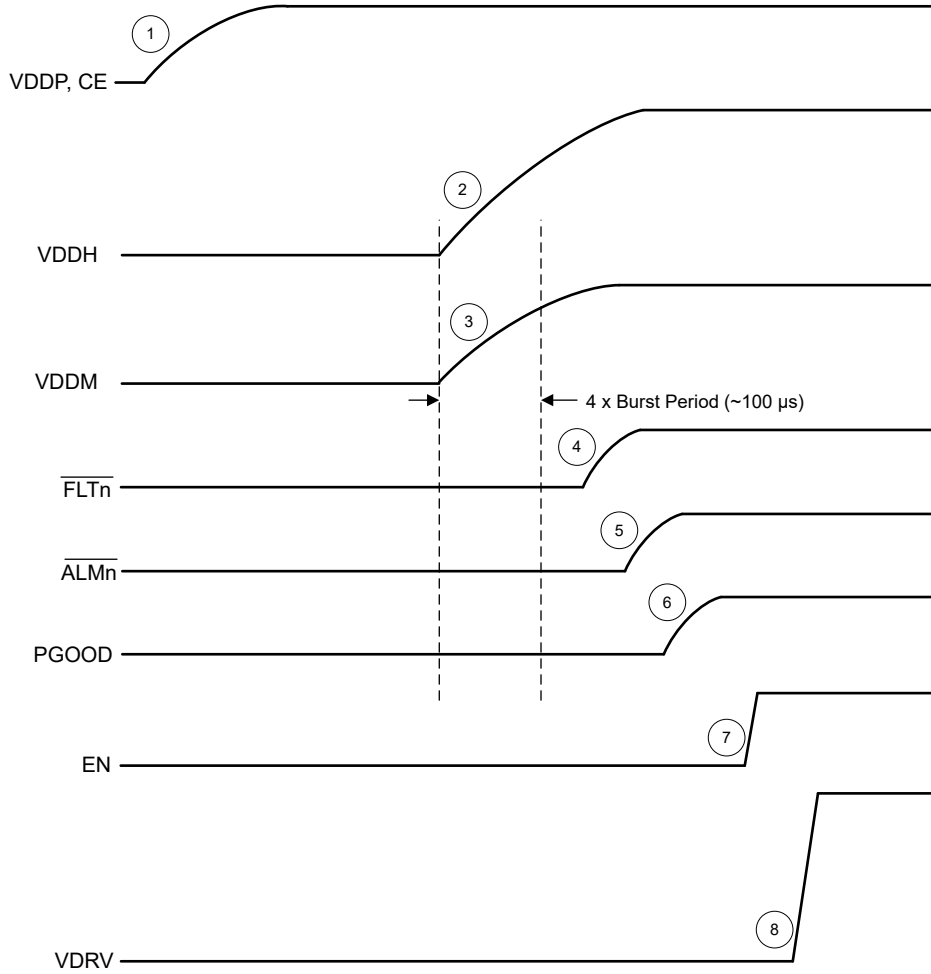
图 8-10. TPSI310x 典型启动 ( CE = VDDP , FLTn_CMP = 0 , ALMn_CMP = 0 )
