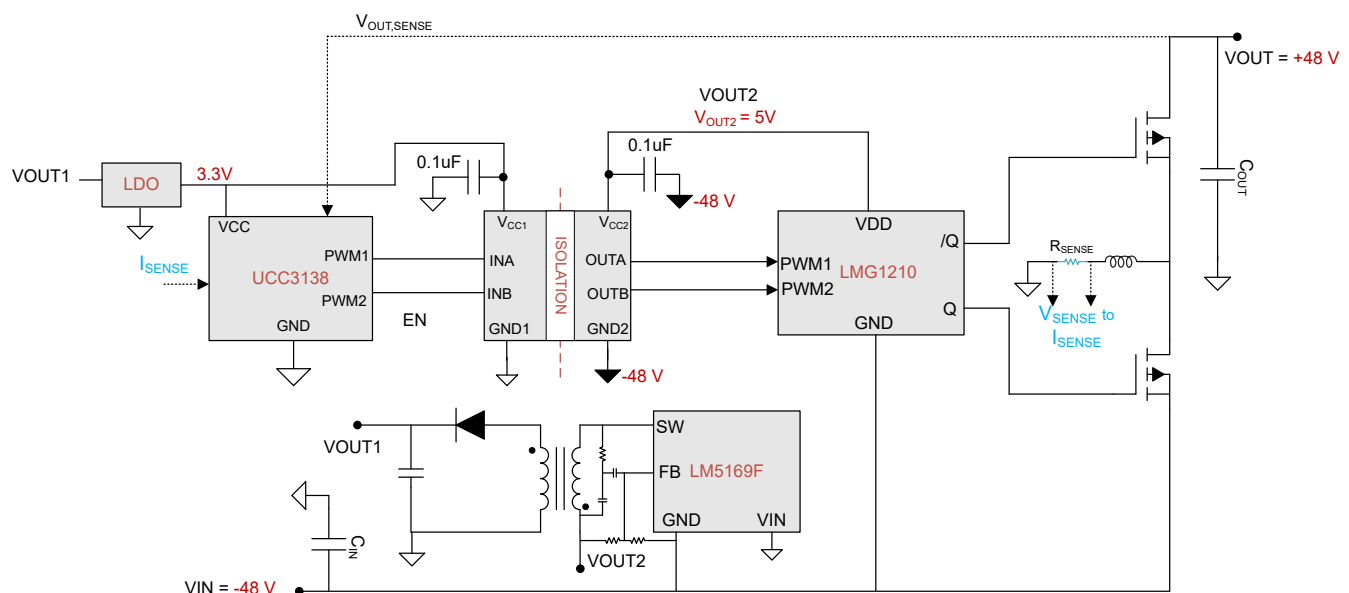
图 8-1. ISO6520 for Level shifting PWM signals from controller referenced to Ground to the FET driver in an Inverted Buck Boost Topology
