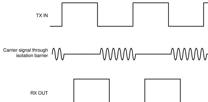
图 7-2. On-Off Keying (OOK) Based Modulation Scheme
