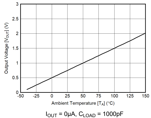
图 5-2. Output Voltage vs Ambient Temperature
