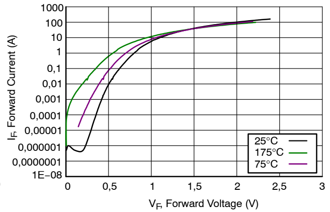
Figure 16. Forward Characteristics
