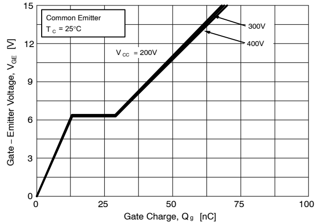
Figure 8. Gate Charge
