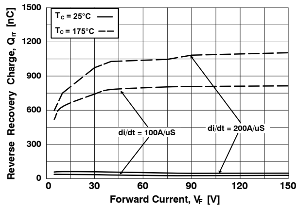
Figure 19. Stored Charge
