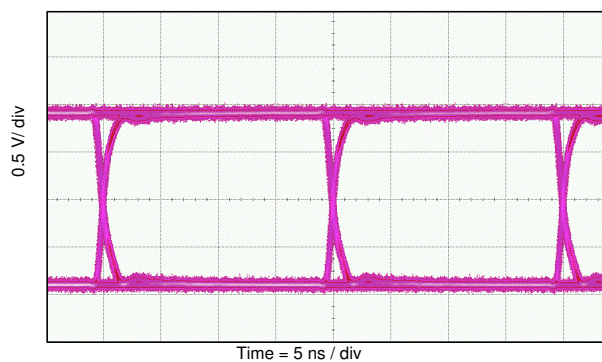
图 9-6. Eye Diagram at 50 Mbps PRBS 2 16 - 1, 1.8 V and 25°C
