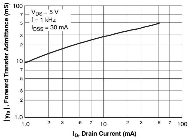
Figure 5. |y_{fs}| - I_D
