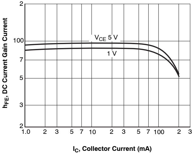
Figure 3. h_{FE} - I_C
