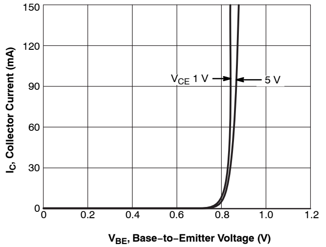
Figure 2. I_C - V_{BE}
