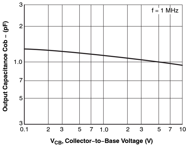
Figure 5. C_{ob} - V_{CB}
