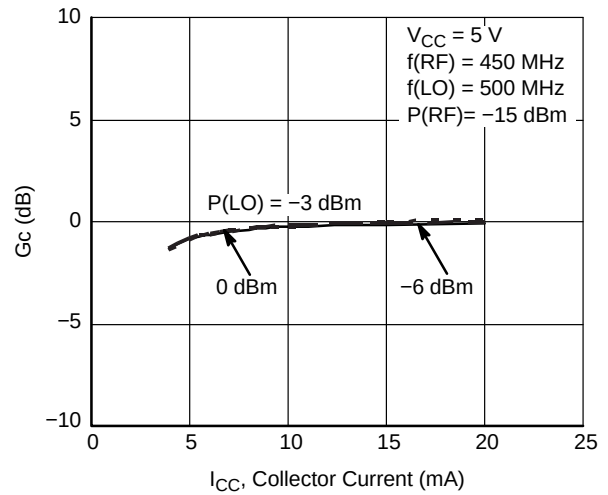
Figure 5. G C – I CC
