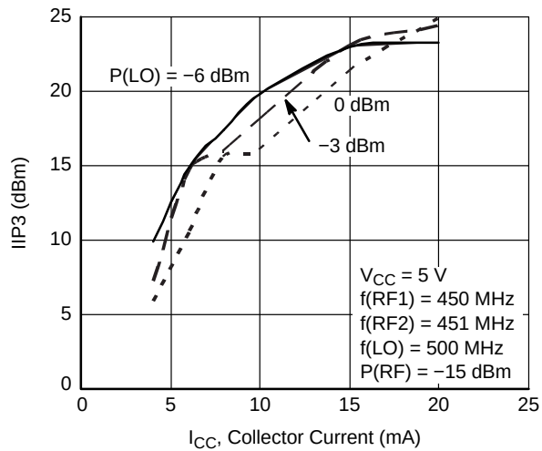
Figure 6. IIP3 – I CC
