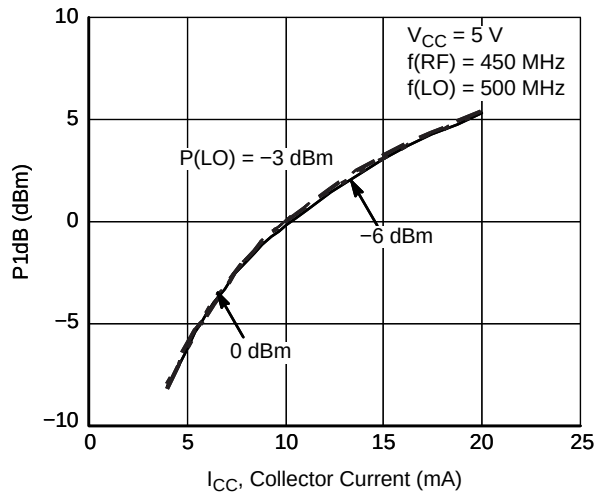
Figure 4. P1dB – I CC
