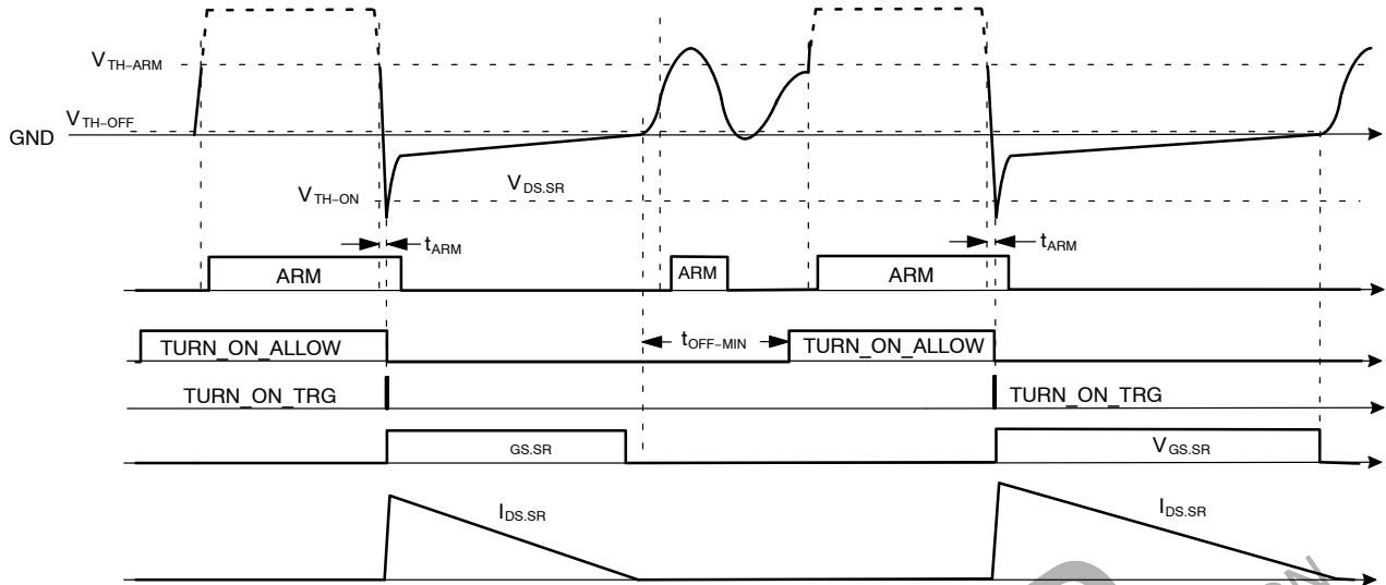
Figure 18. SR Turn-On Algorithm
