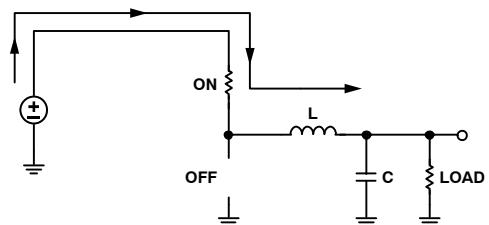
Figure 18. Buck Topology Inductor Current During t_0 and t_1
