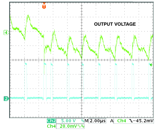
Figure 10. Load Transient, 3 A to 10 A, V_{IN} = 12\text{ V}
