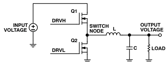
Figure 17. Buck Topology
