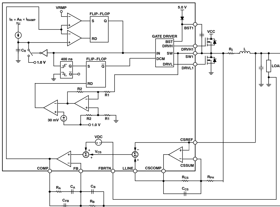
Figure 13. RPM Mode Operation
