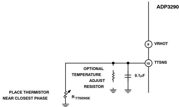
Figure 14. VR Thermal Monitor Circuit
