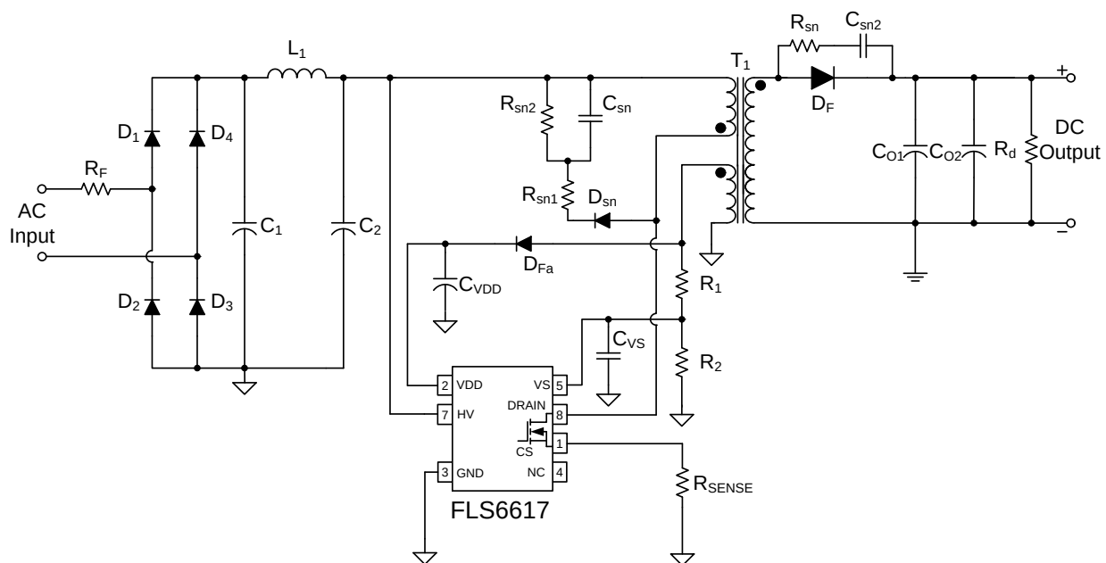
Figure 2. Application Diagram
