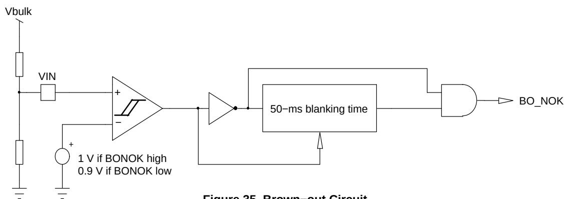
Figure 35. Brown-out Circuit
