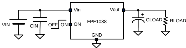
Figure 28. Device Setup
