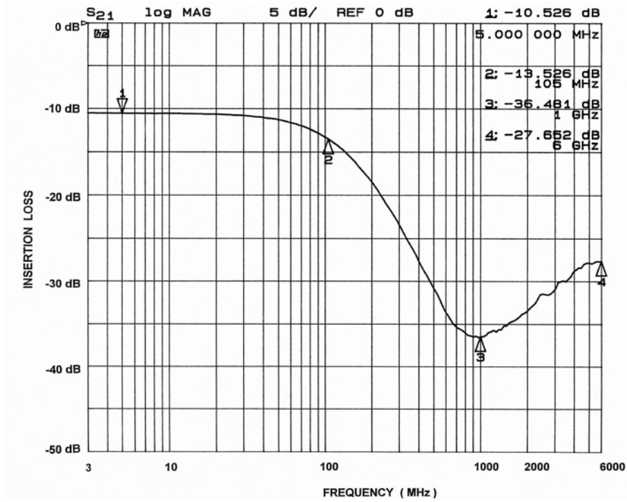
Figure 1. Channel 1 EMI Filter Performance
