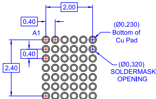
RECOMMENDED LAND PATTERN (NSMD TYPE)
