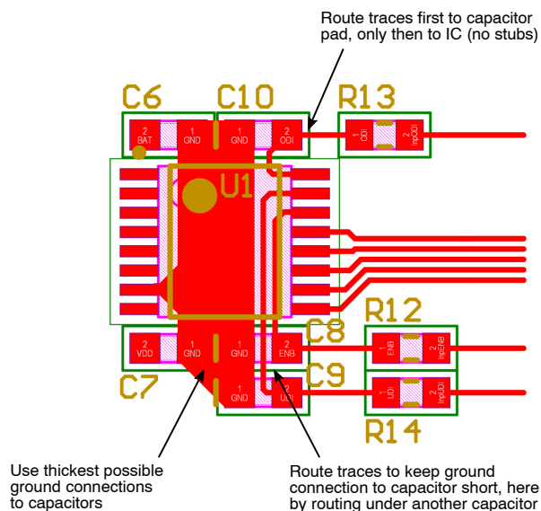
Figure 9. Possible Single-Layer Layout for ODI, UDI, and ENB Decoupling
