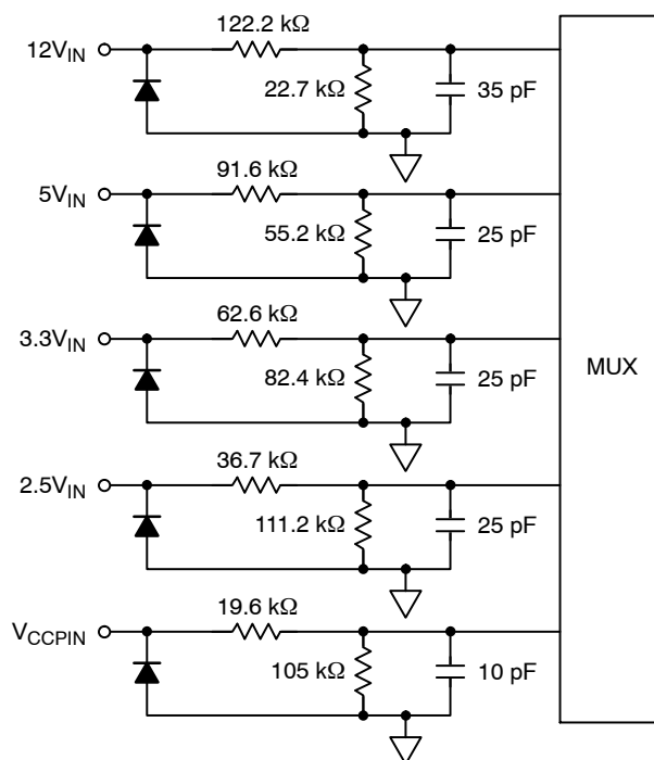
Figure 13. Structure of Analog Inputs
