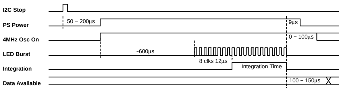
Figure 14. Proximity Sensor One-Shot Timing
