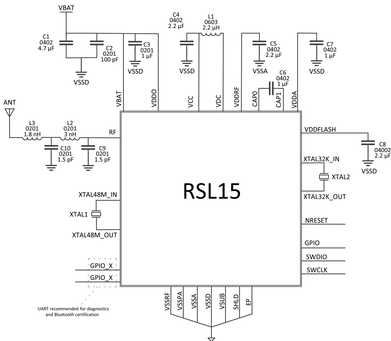
Figure 6. RSL15 BUCK Mode Connection Diagram, VDDO = VBAT
