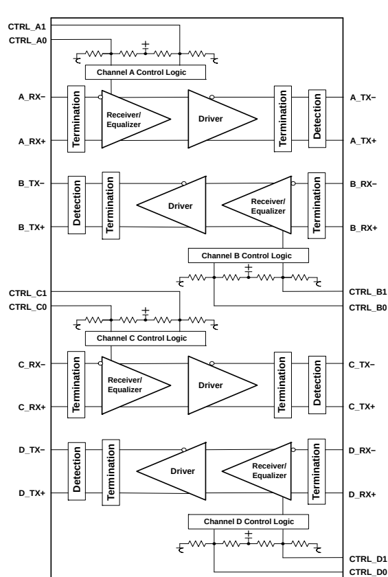
Figure 1. Logic Diagram
