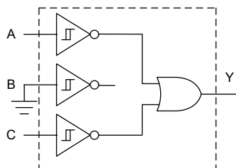
2 - Input OR Gate
