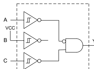
2 - Input AND Gate with inverted input (A)
