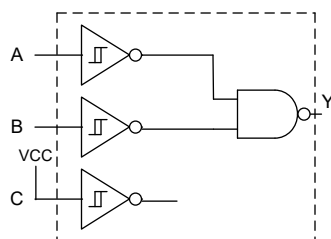
2 - Input NAND Gate
