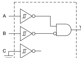
2 - Input AND Gate with inverted input (B)
