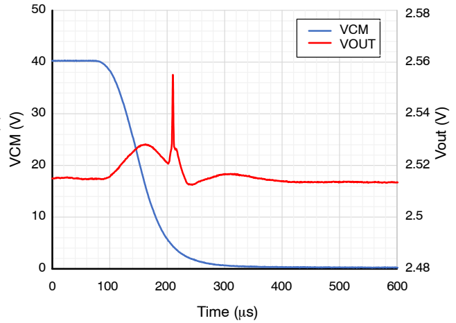
Figure 23c. Common Mode Voltage Step Falling, G100 (10μs)
