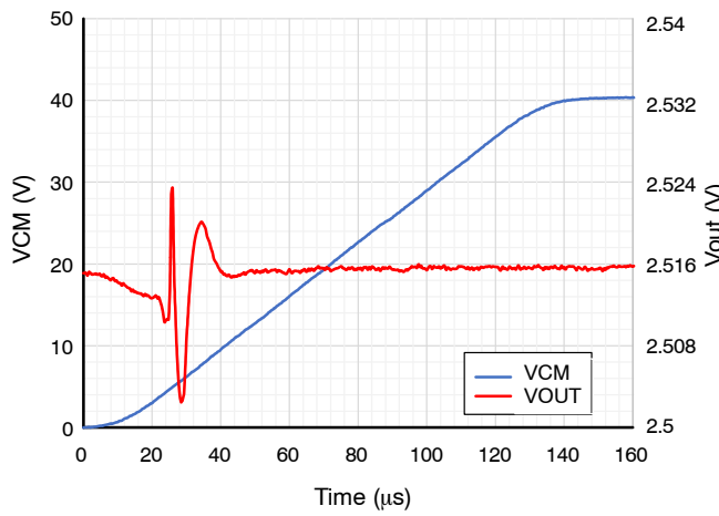
Figure 23b. Common Mode Voltage Step Rising, G100 (100μs)
