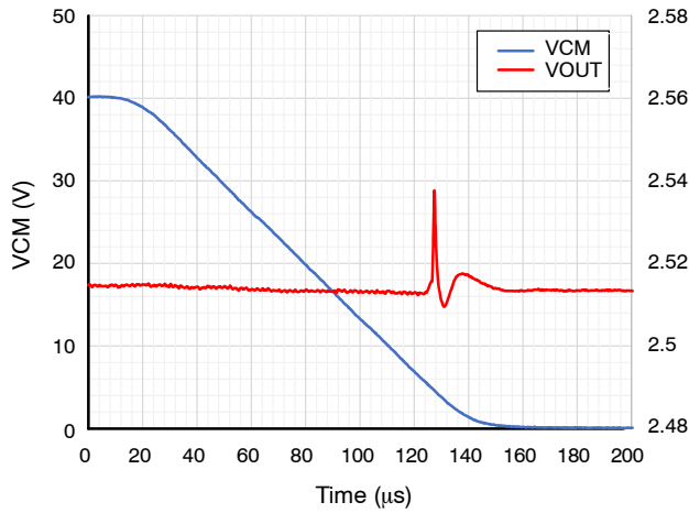
Figure 23d. Common Mode Voltage Step Falling, G100 (100μs)
