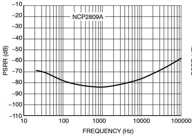
Figure 30. PSRR – Input Grounded with 10 \Omega V_p = 3.3 V, V_{\text{ripple}} = 200 mV pk-pk, R_L = 16 \Omega
