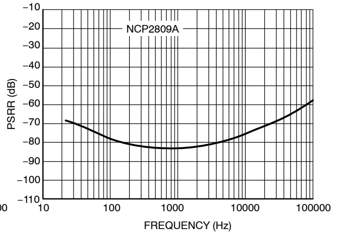
Figure 31. PSRR – Input Grounded with 10 \Omega V_p = 3.3 V, V_{\text{ripple}} = 200 mV pk-pk, R_L = 32 \Omega
