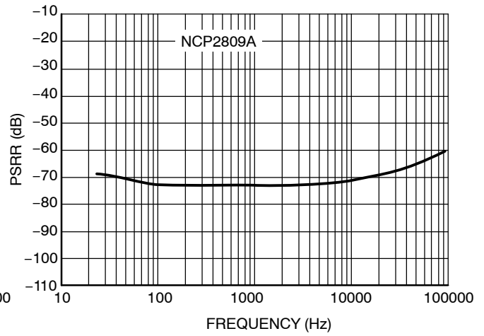
Figure 33. PSRR – Input Grounded with 10 \Omega V_p = 5.0 V, V_{\text{ripple}} = 200 mV pk-pk, R_L = 32 \Omega
