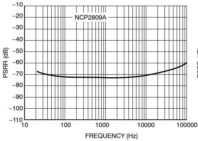
Figure 32. PSRR – Input Grounded with 10 \Omega V_p = 5.0 V, V_{\text{ripple}} = 200 mV pk-pk, R_L = 16 \Omega
