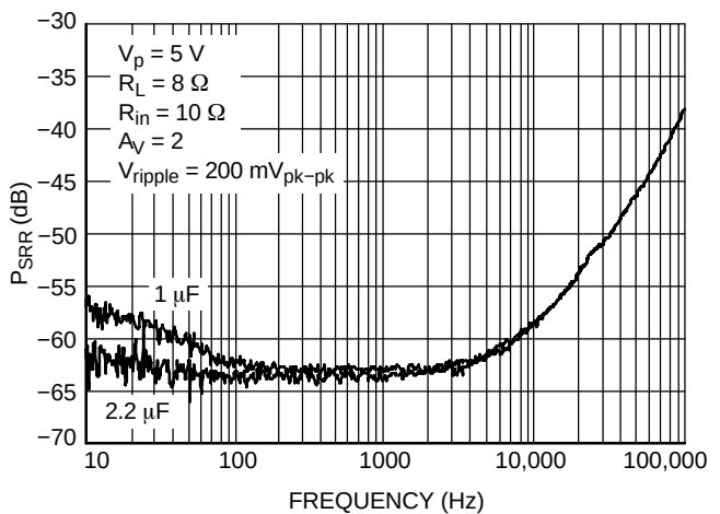
Figure 24. P_{SRR} versus C_{bypass} @ V_p = 5 V
