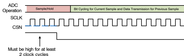
Figure 17. SAR ADC Internal Operation
