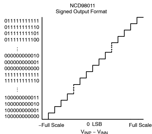
Figure 19. NCD98011 Signed Output Definition
