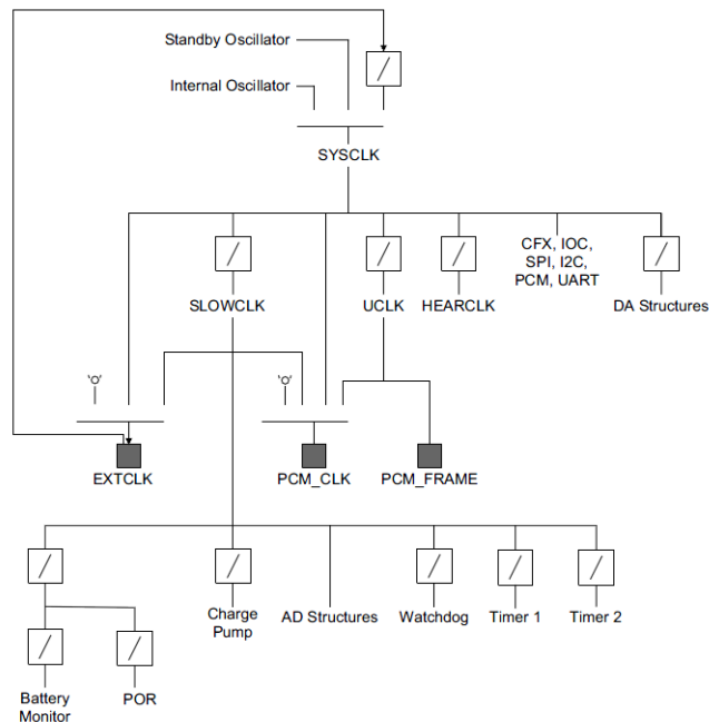
Figure 12. Internal Clocking Structure
