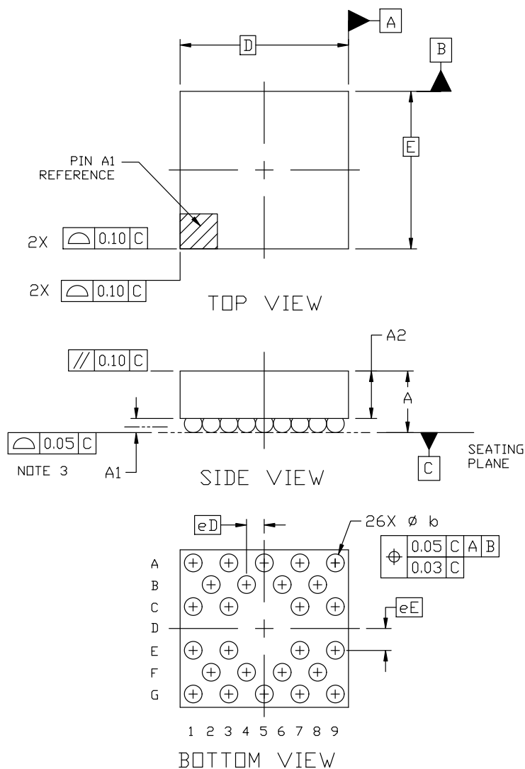
WLCSP26, 2.388x2.233 CASE 567CY ISSUE B
