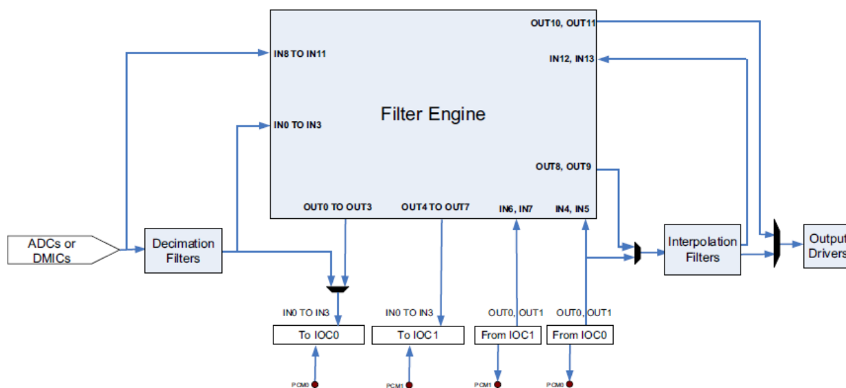
Figure 3. Filter Engine: Audio Filtering and Multiplexing
