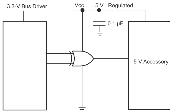
图 8-1. Typical Application Schematic
