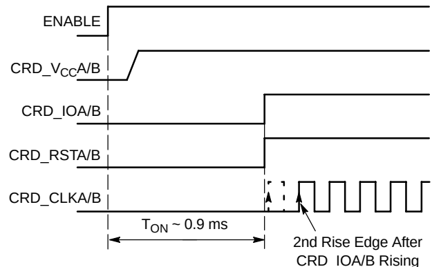
Figure 12. NCN4557 Power-Up
