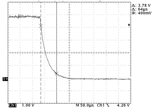
Typical CRD_VCC Fall Time @ Cout = 10 μF, V = 5.0 V
