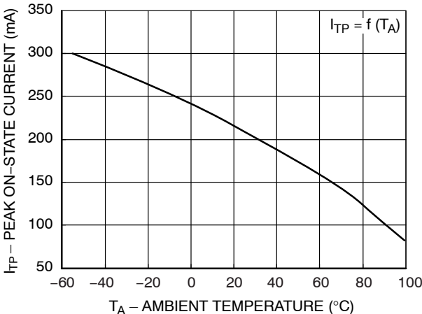
Figure 11. Current Reduction
