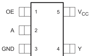
图 4-1. SN74LV1T126-Q1 DCK or DBV Package, 5-Pin SC70 or SOT-23 (Top View)
