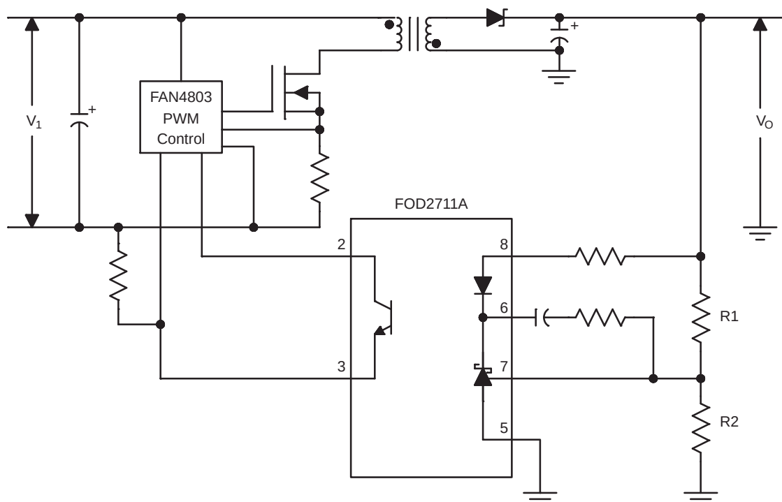
Figure 1. Typical Application
