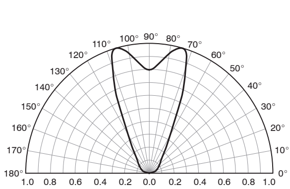
Figure 7. Radiation Diagram
